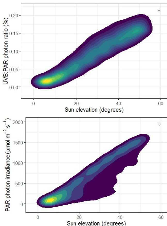
Figure 2 A. Photon ratio between the UV-B and PAR components of sunlight, and B. PAR photon irradiance, both as a function of solar elevation (degrees above the horizon). Contours represent the density of data points, computed from 11 768 hourly solar spectra for Helsinki, Finland, 1 st May - 30 th September 2013-2017 (Anders Lindfors and Pedro J Aphalo, unpublished simulated spectral data and its analysis respectively).
